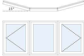
3 Unit Bow Window 15°
