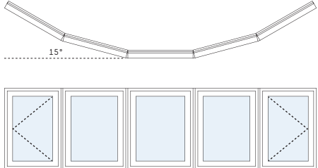
5 Unit Bow Window 15°
