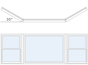
3 Unit Bay Window 30°
