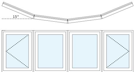
4 Unit Bow Window 15°
