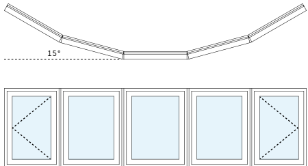
5 Unit Bow Window 15°
